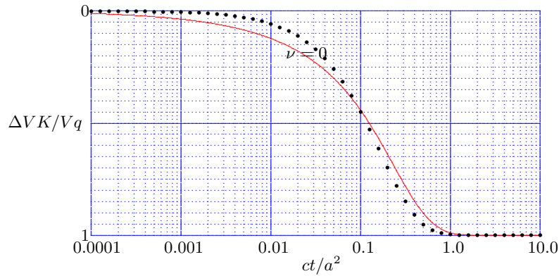
Figure 3.22: Cryer's problem : Volume change and approximation.
