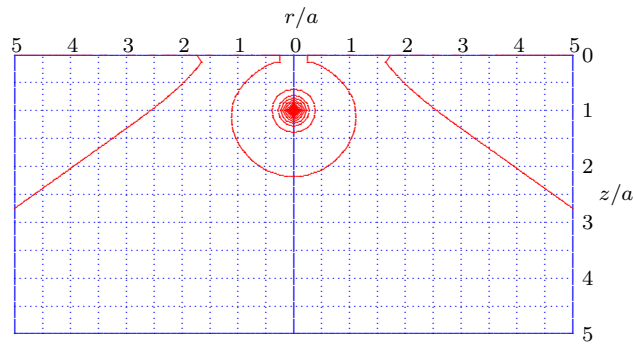
Figure 5.22: Pore pressure distribution, for c_v t/h^2 = 0.1 .
