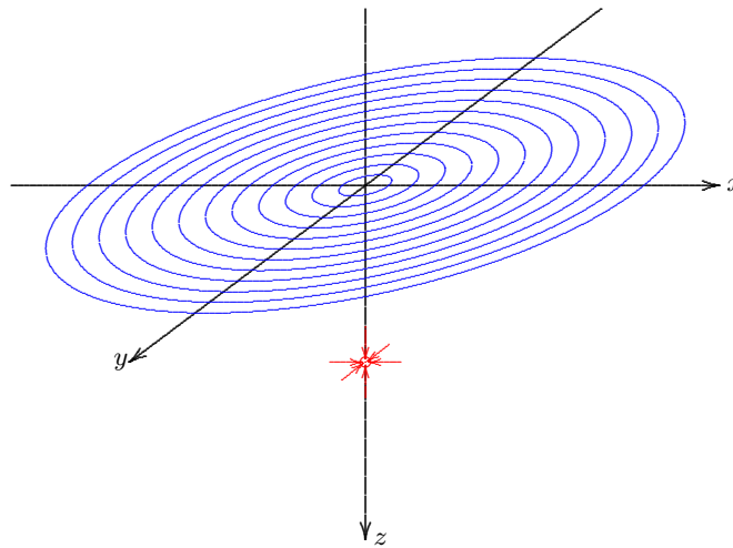
Figure 5.18: Point sink in half space.
