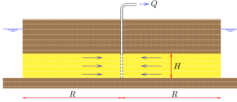
Figure 5.11: A well in a finite confined aquifer, Plane stress model.
