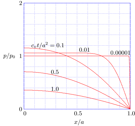
Figure 3.3: Pore pressure distribution for Mandel's problem, \nu = 0.0 .
