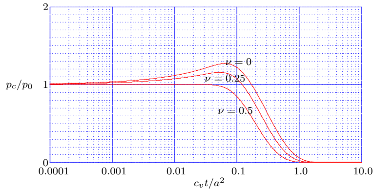
Figure 3.9: De Leeuw's problem : Pore pressure in the center.
