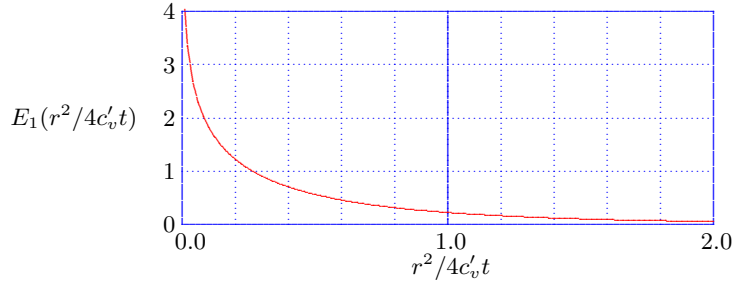
Figure 5.9: Exponential Integral.
