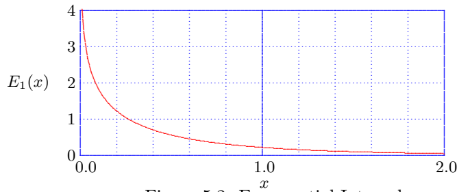
Figure 5.2: Exponential Integral.
