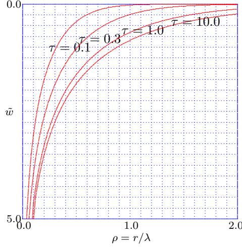
Figure 5.15: Leaky aquifer : vertical displacement.
