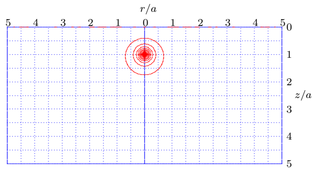
Figure 5.24: Pore pressure distribution, for c_v t/h^2 = 1000 .
