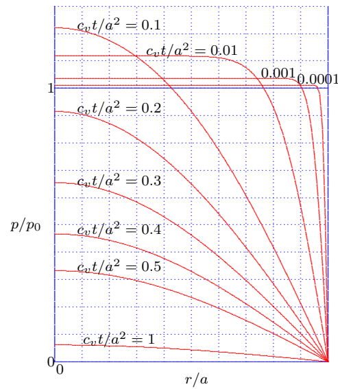
Figure 3.10: De Leeuw's problem : Pore pressures.
