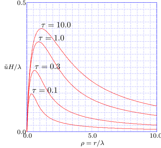
Figure 5.16: Leaky aquifer : radial displacement.
