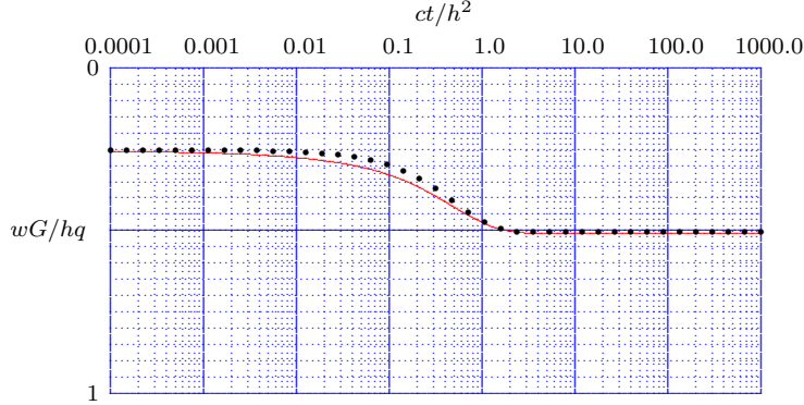
Figure 3.20: PSPL : Surface displacement.
