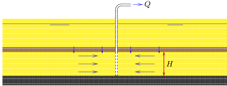
Figure 5.14: A well in a leaky aquifer.
