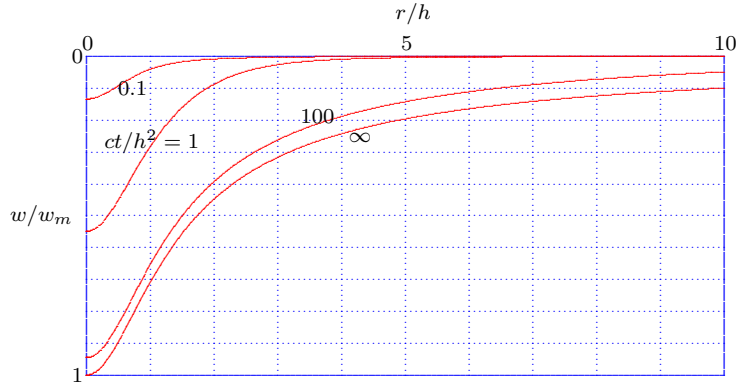
Figure 5.21: Vertical displacement of surface, for c_v t / h^2 = 0.1, 1, 100, \infty .
