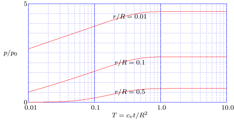
Figure 5.8: Finite Aquifer : Pore pressure as a function of T , Theis-Jacob model.
