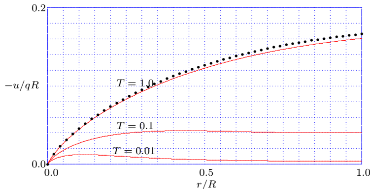
Figure 5.12: Well in finite aquifer, Plane stress model : Horizontal displacement.
