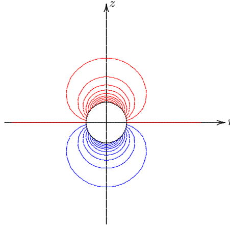
Figure 3.18: Spherical inclusion, contours of initial pore pressure.
