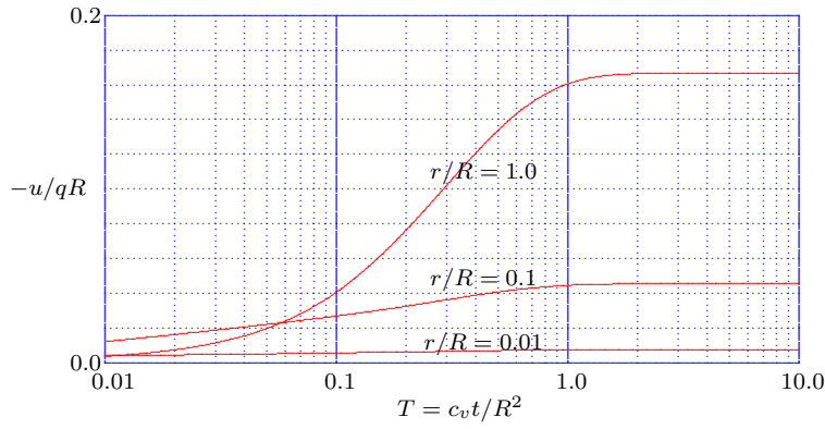
Figure 5.13: Well in finite aquifer, Plane stress model : Horizontal displacement.
