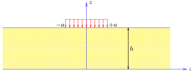
Figure 3.19: Strip load on poroelastic layer.
