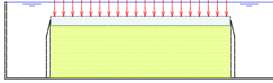
Figure 2.8: One-dimensional consolidation with periodic load.
