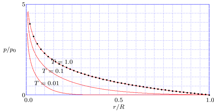
Figure 5.7: Finite aquifer : Pore pressure as a function of r/R , Theis-Jacob model.
