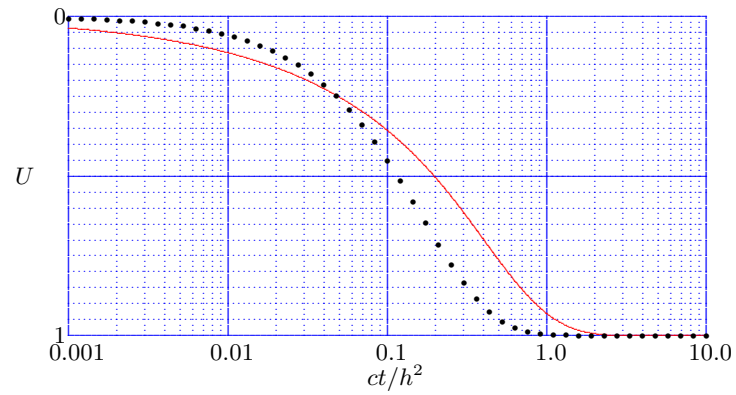
Figure 3.23: Terzaghi's problem : Degree of Consolidation.
