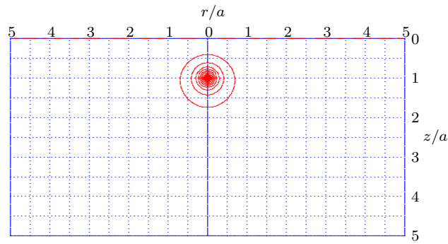
Figure 5.23: Pore pressure distribution, for c_v t/h^2 = 10 .
