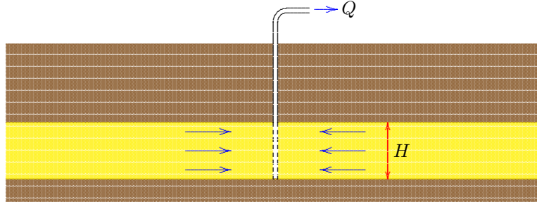
Figure 5.1: Well in infinite confined aquifer, Theis-Jacob model.
