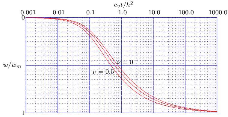
Figure 5.20: Vertical displacement of surface, for r/h = 0 , \nu = 0, 0.25, 0.5 .
