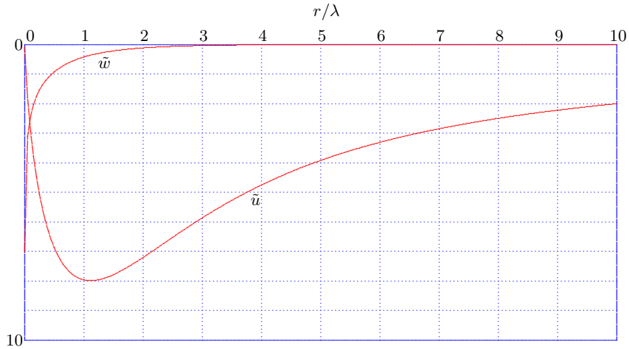
Figure 5.17: Radial and vertical displacements in a leaky aquifer, \lambda/H = 20 .
