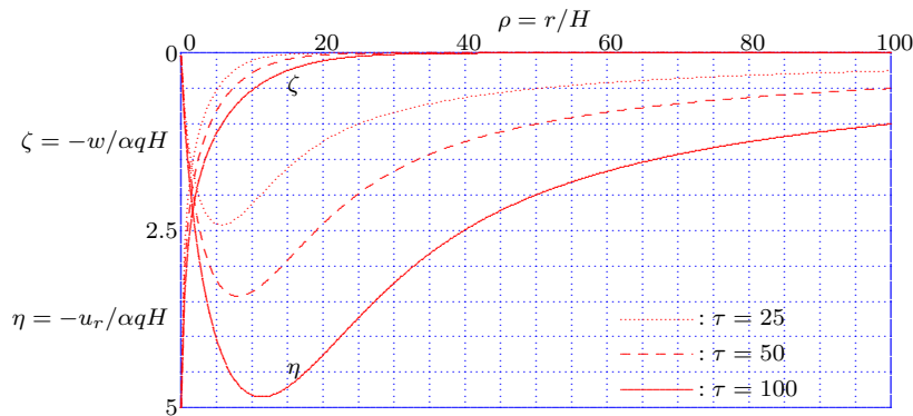
Figure 5.10: Well in infinite aquifer, Plane stress model : displacements.
