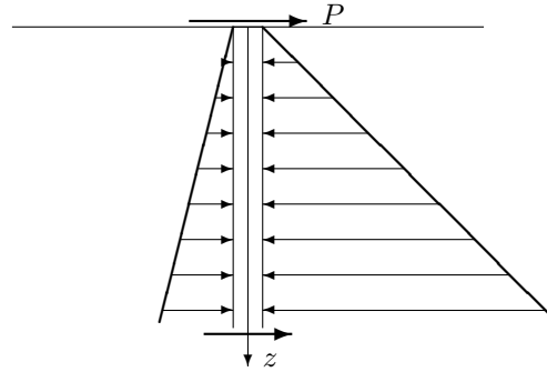
Figure 8.5: Soil reaction according to Blum.
